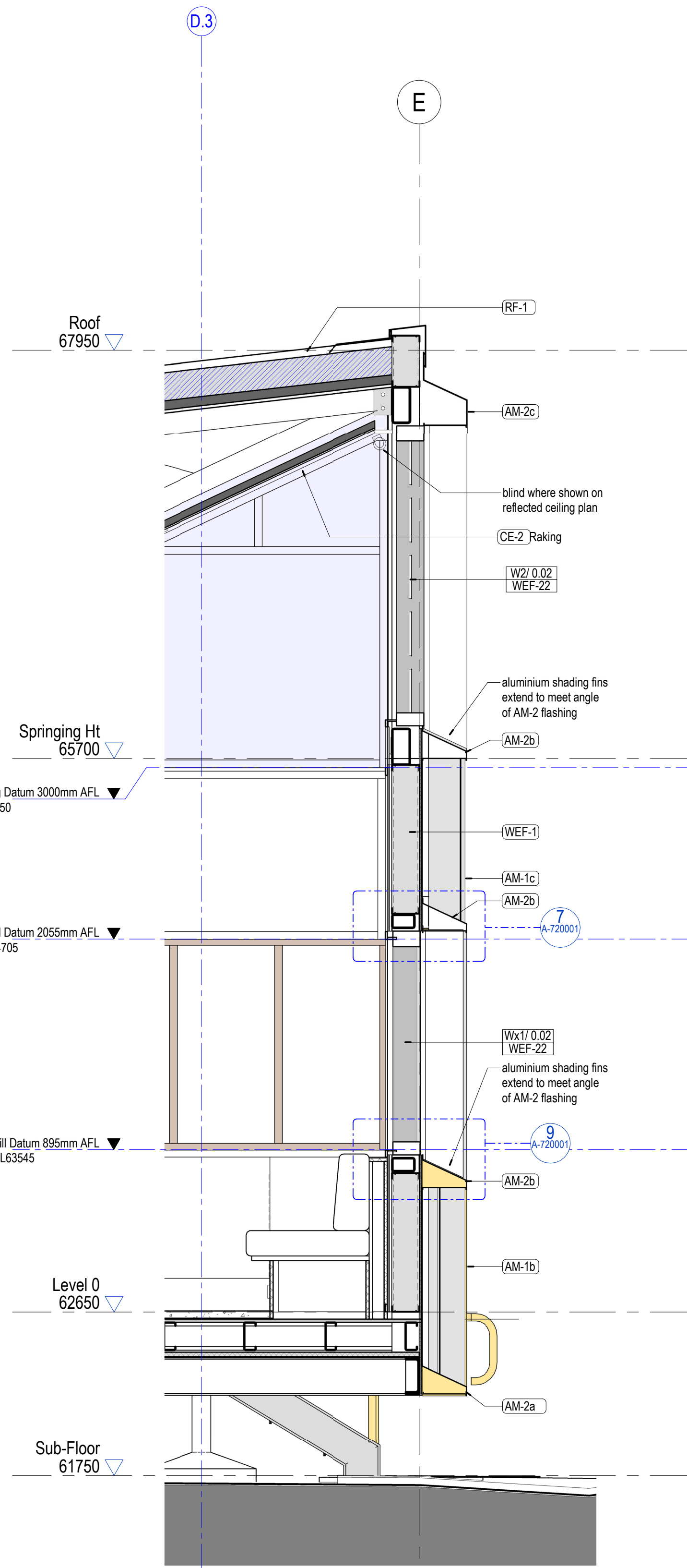
1 East Low + High Window Section 1 : 20 Covered Outdoor
