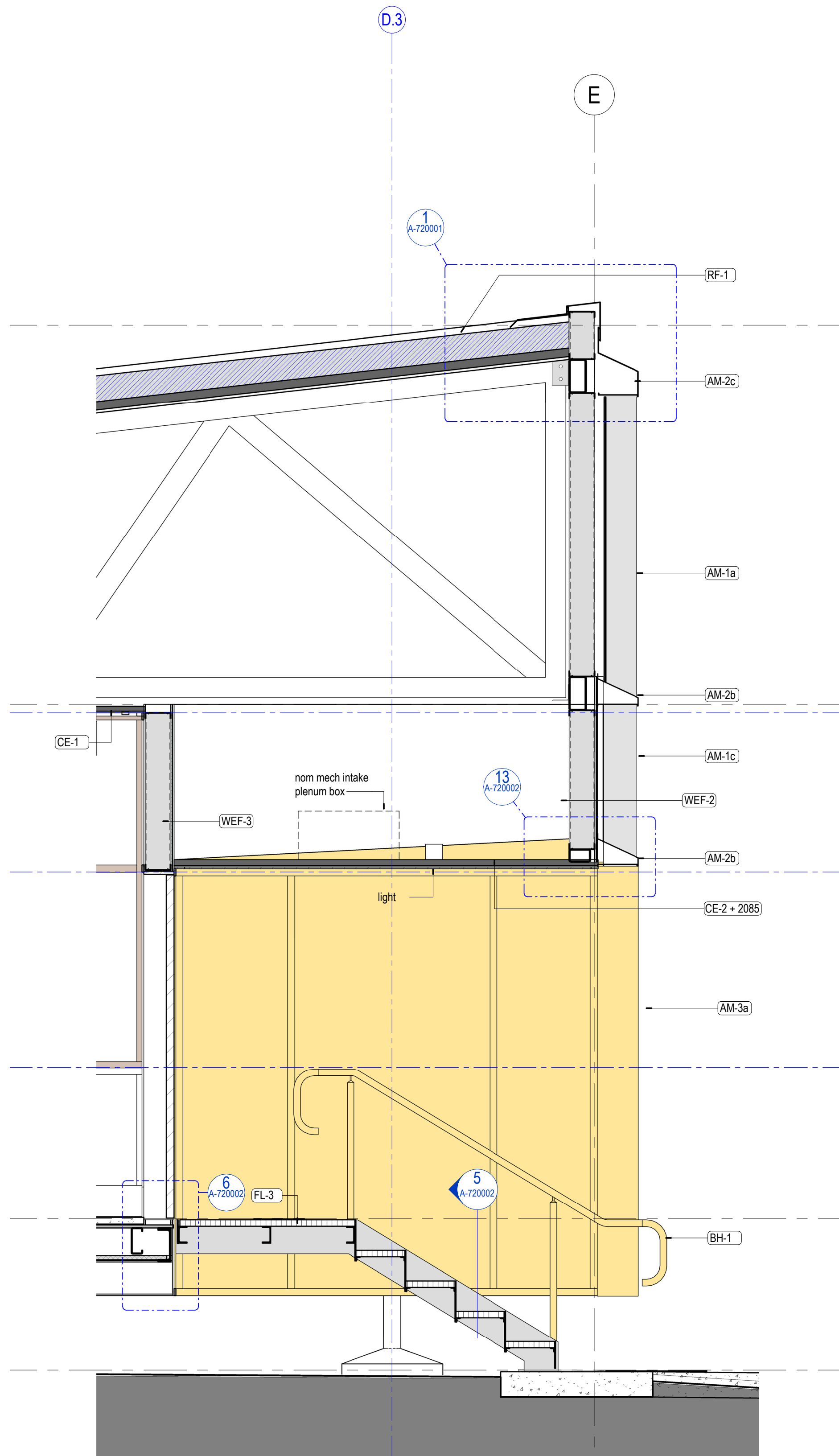
2 East Stair 1 Facade Section 1 : 20 Covered Outdoor
