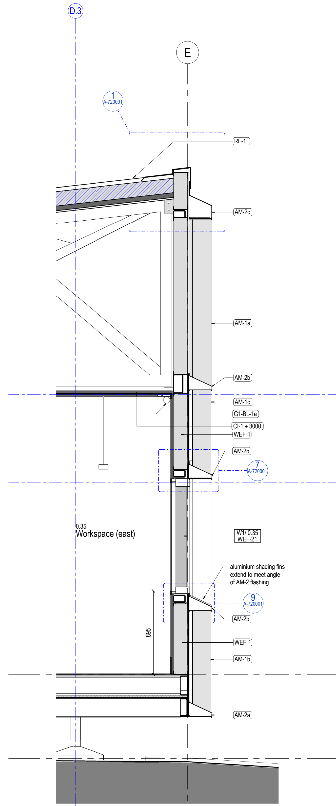
3 East Low Window Section 1 : 20 Typ Low Window
